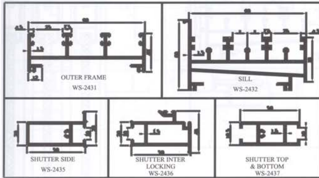
EXTRUDED PROFILES
