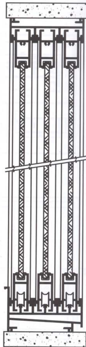
SECTION-BB
