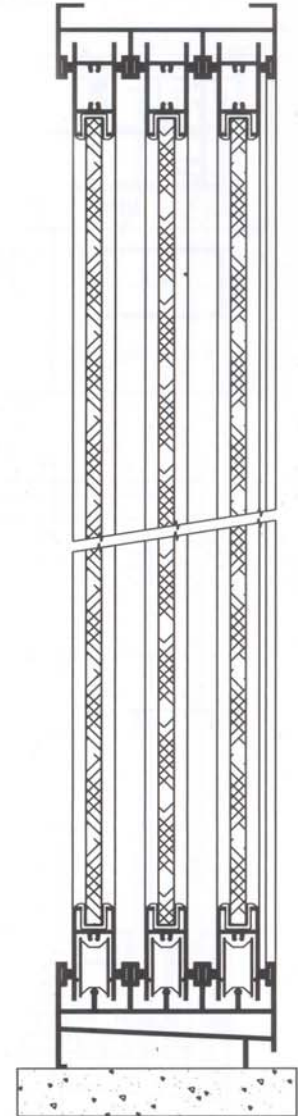
SECTION-BB
