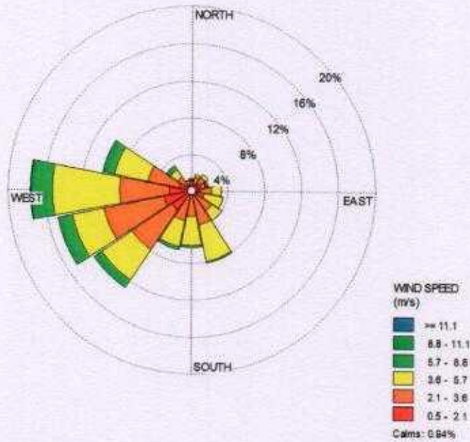
Figure.01: Wind Rose Diagram (July-August-Sept-2021)
