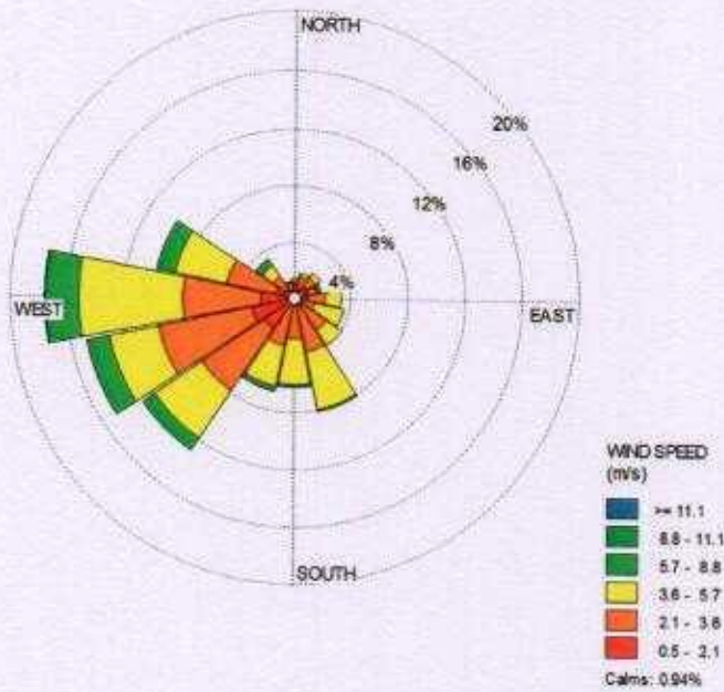
Figure.01: Wind Rose Diagram (July-August-Sept-2021)
